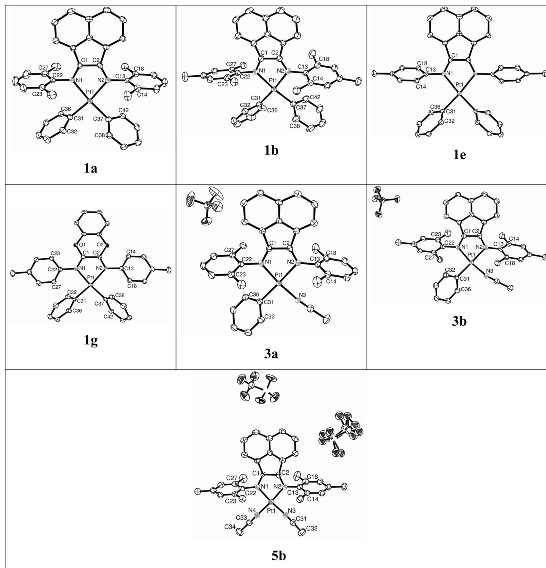
Figure 1. ORTEP drawings of (N–N)Pt II complexes 1a , 1b , 1e , 1g , 3a–b , and 5b . 50% probability ellipsoids are shown (hydrogen atoms are removed for clarity). In 5b there are two molecules in the asymmetric unit, but only one is shown for clarity).
