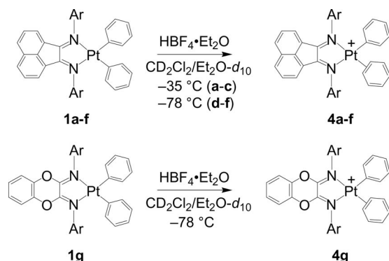
Scheme 4.
